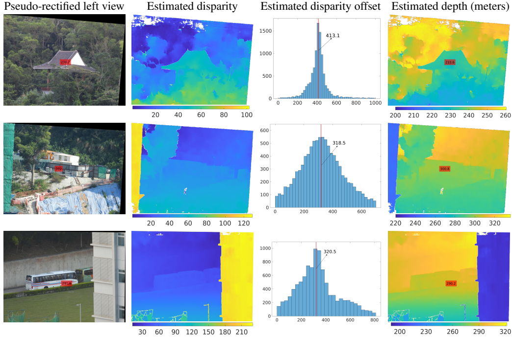
Figure 10: Results on real-world data. The depth measurements from a laser rangefinder are marked in the red box on the pseudo-rectified left images; the corresponding estimated values by our method are marked on the estimated depth maps. Laser-measured values (top to bottom): 234.2m, 302m, 291.9m; our estimated values (top to bottom): 233.6m, 300.8m, 290.2m.
