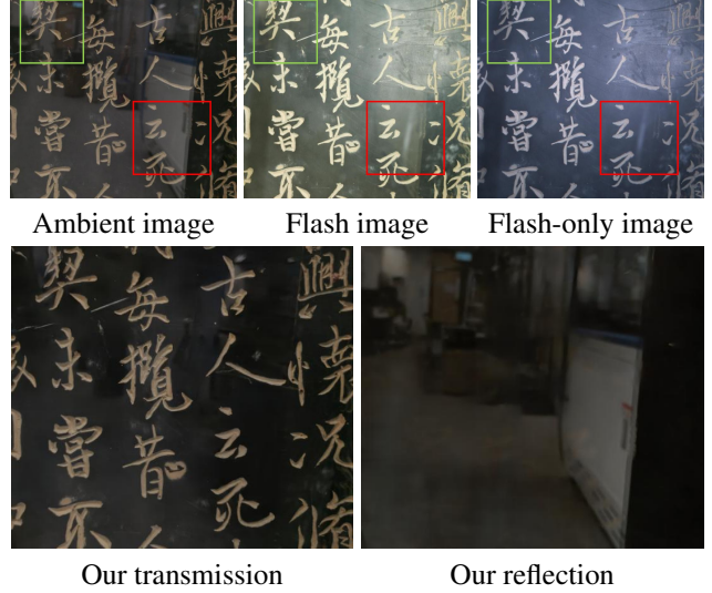
Figure 1. A reflection-free flash-only image is computed from a pair of ambient/flash images to help remove reflection. Our transmission image does not absorb the artifacts in the flash-only image.
