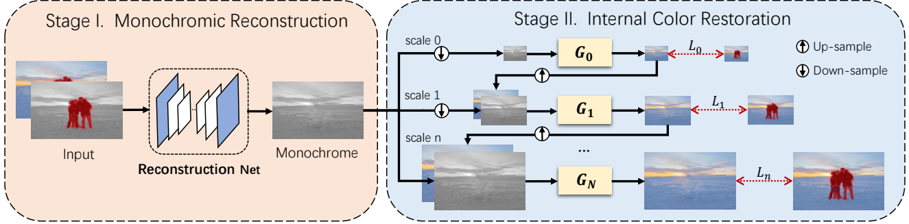
Figure 2. Overview of our external-internal inpainting method. It externally learns to reconstruct structures in the monochromatic space via training on large datasets, while implicitly propagates colors within the single test image via internal learning. The colorization loss L_n is only calculated on the unmasked regions.
