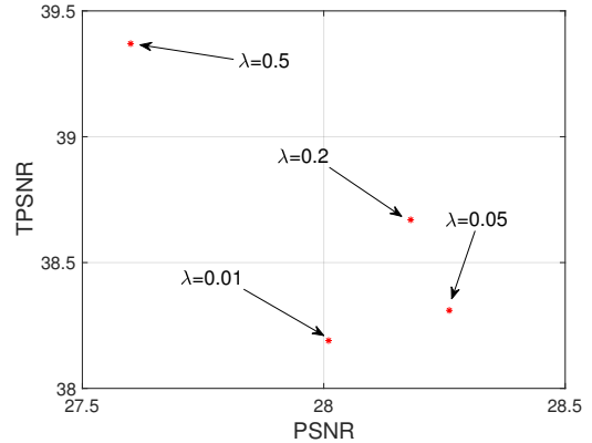
Figure 7. The parameter \lambda trades off spatial and temporal accuracy.
